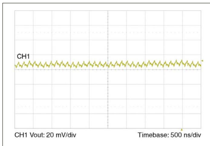
Figure 6 — Output voltage ripple at full load and 48 Vf with 3.3 \mu F ceramic POL bypass capacitance and 20 nH distribution inductance.
