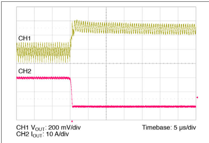
Figure 13 – 20 A – 0 A transient response; C_{IN} = 100 \mu F , no external C_{OUT}
