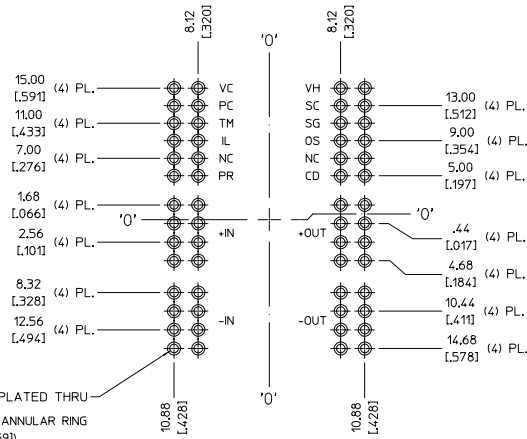
RECOMMENDED LAND PATTERN (COMPONENT SIDE SHOWN)
