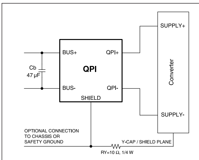
Figure 1 - QPI-4 circuit on input bus.
