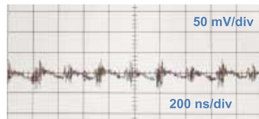
4(b) Vicor 3.5 MHz Bus Converter
