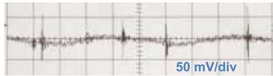
5(a) 100 kHz PWM Forward
