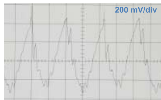
4(c) IR's Half Bridge Bus Converter (Note different scale)
