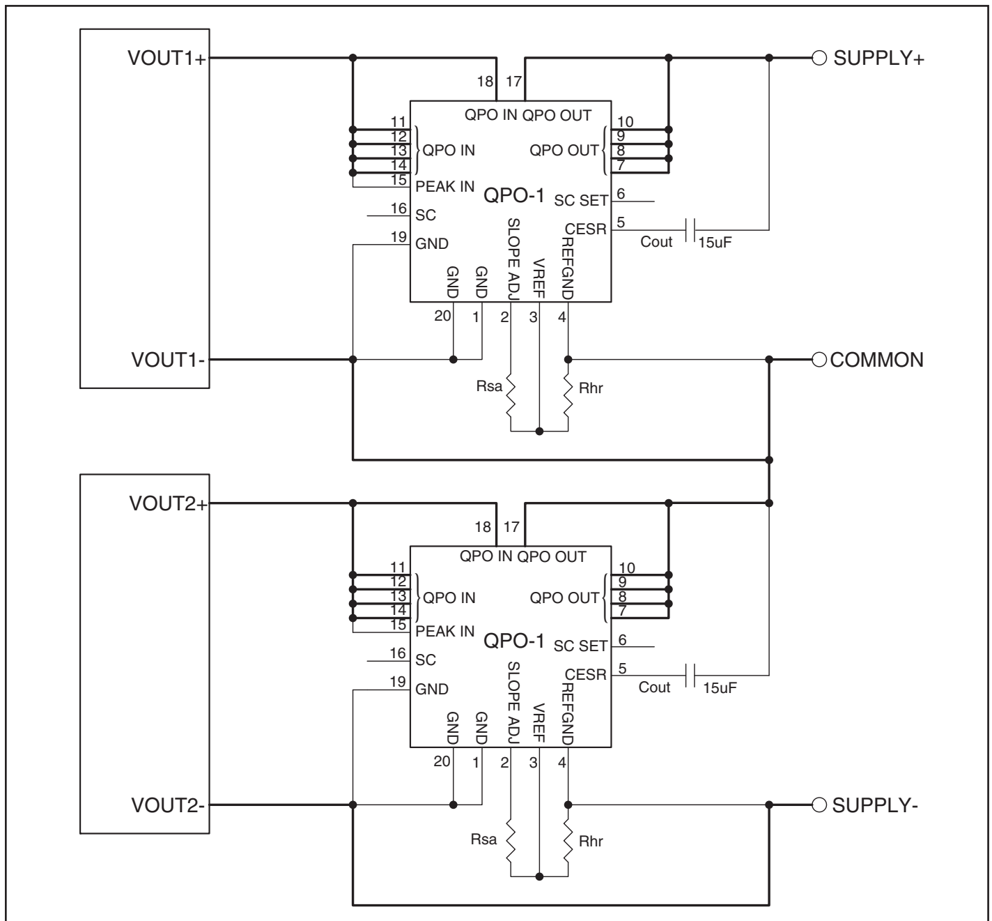
Figure 12- Schematic for +/- supply application. Circuit shown is for an open loop configuration. See text and schematic showing SC/Trim and remote sense application if required. Dark lines show high-current path.
