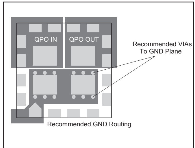
Figure 15 - Recommended copper pattern for LGA mounting showing QPO pads and minimum copper landing. Pattern should be on 2 oz. copper with vias, placed outside of device pad solder mask openings, used to connect to internal layers (if required).
