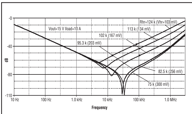
Figure 7 – Attenuation at different headroom settings with 25 \mu F capacitor connected to V_{ref} .
